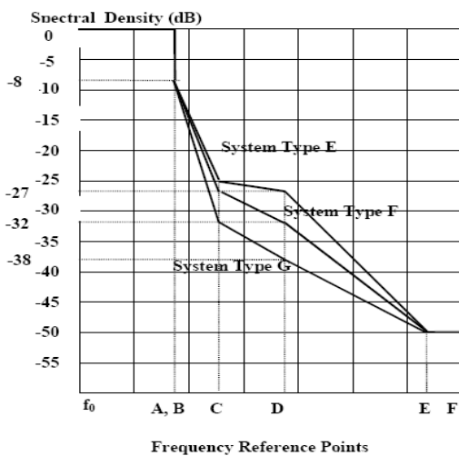
Figure 3. WiMAX Spectral Emission Mask
