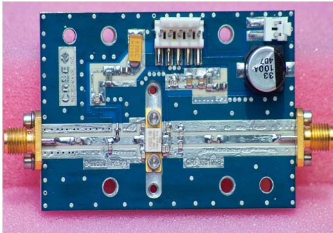
Figure 1. CRF35010 and test board
