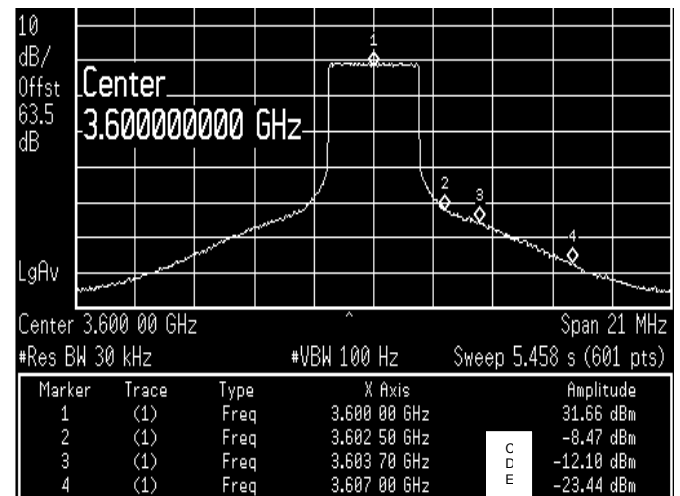
Figure 4. Spectral plot of CRF35010 at 1.5W Average, 3.6GHz
