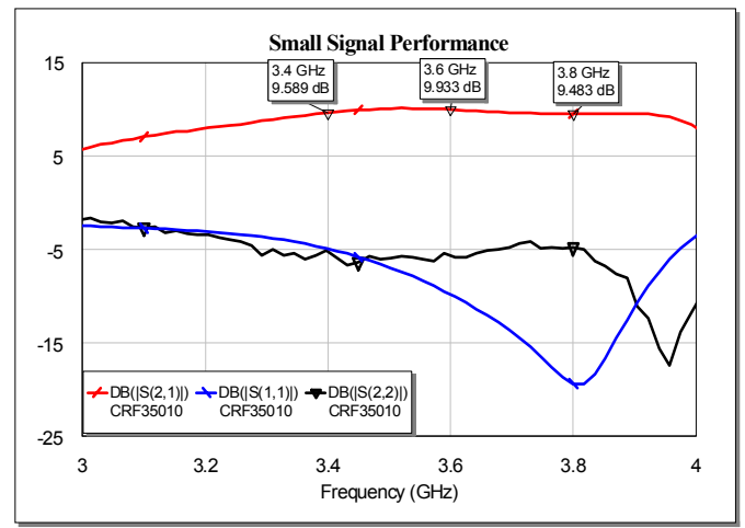
Figure 2. Small signal s-parameters of CRF35010 in test board
