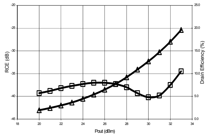
Figure 6. RCE and Drain Efficiency vs Average Output Power for CRF35010 at 3.6GHz
