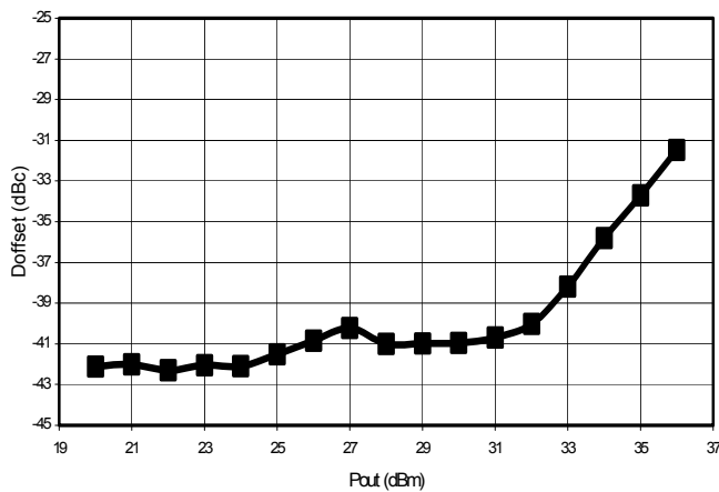
Figure 5. WiMAX Relative Offset Power vs Average Output Power for CRF35010 at 3.6GHz
