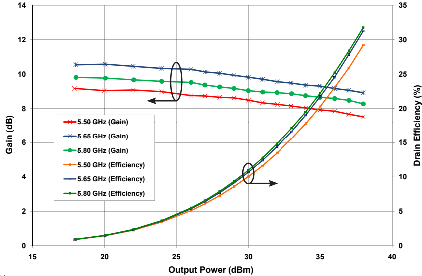
Drain Efficiency and Gain vs Output Power of CGH55030F in CGH55030F-TB V_{DD} = 28\text{ V} , I_{DQ} = 250\text{ mA} , 802.16-2004 OFDM, PAR=9.8 dB
