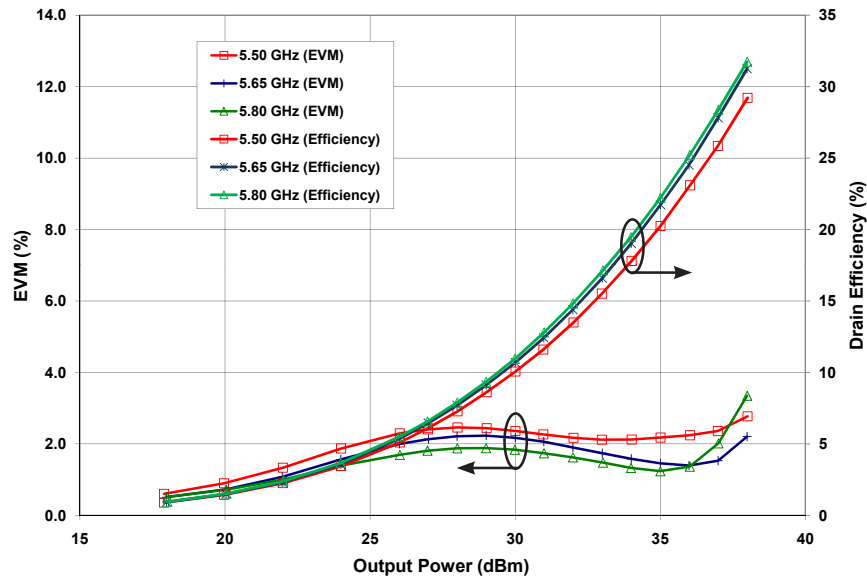
Typical EVM and Drain Efficiency vs Output Power of CGH55030F in CGH55030F-TB at 5.50GHz, 5.65 GHz, 5.80GHz, 802.16-2004 OFDM, PAR=9.8 dB
