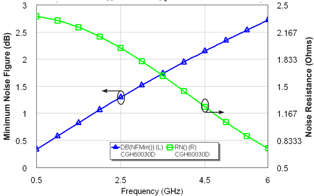
Simulated Minimum Noise Figure and Noise Resistance vs Frequency of the CGH60030D V_{DD} = 28\text{ V} , I_{DQ} = 250\text{ mA}
