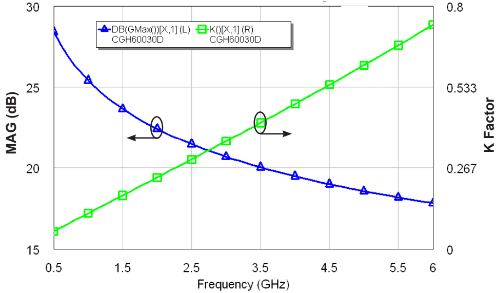
Simulated Maximum Available Gain and K Factor of the CGH60030D V_{DD} = 28\text{ V} , I_{DQ} = 250\text{ mA}
