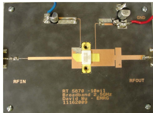
Fig. 6. Fabricated input and output matching network
