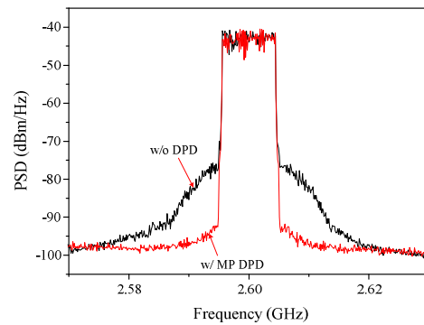
Fig. 9. Output spectrum before and after linearization for 10 MHz LTE signal at 2.6 GHz
