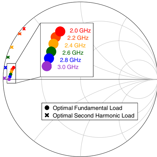
Fig. 1. Optimal fundamental and second harmonic load impedance derived from loadpull at the device package plane
