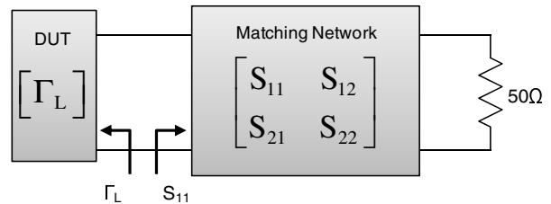
Fig. 3. Matching an arbitrary load to a resistive termination
