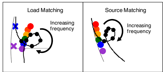
Fig. 5. SRFT generated fundamental impedances vs. optimum matching in Fig. 1 and Fig. 2
