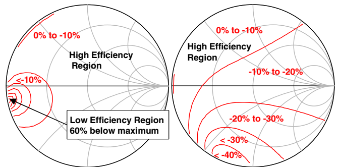
Fig. 4. Second harmonic load pull PAE contours at 2f_0=4.0GHz (left) and 2f_0=6.0GHz (right) indicating drain efficiency percentage below maximum in different regions of the Smith chart.
