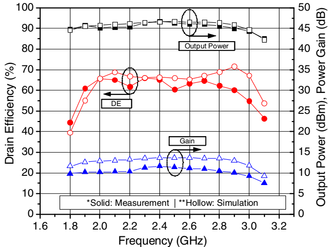
Fig. 7. Measurement versus simulation results showing drain efficiency, output power, and gain from 1.8 GHz to 3.1 GHz
