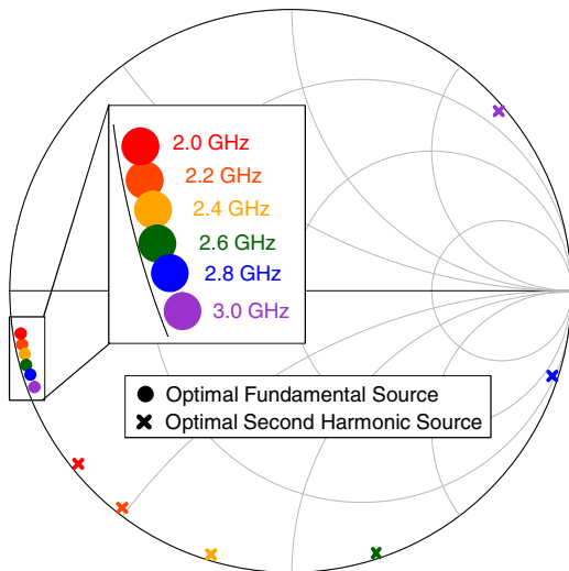
Fig. 2. Optimal fundamental and second harmonic source impedance derived from sourcepull at the device package plane
