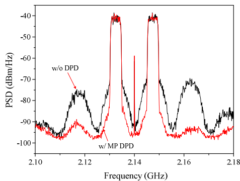
Fig. 8. Output spectrum before and after linearization for 1001 WCDMA signal at 2.14 GHz
