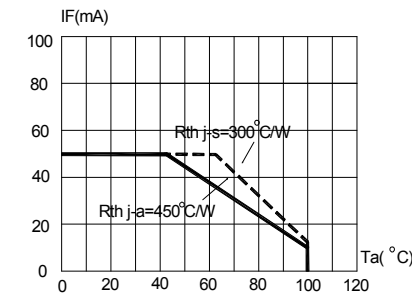
FIG.4a RED MAXIMUM FORWARD DC CURRENT VS AMBIENT TEMPERATURE ( T_{jmax}=110^{\circ}C )
