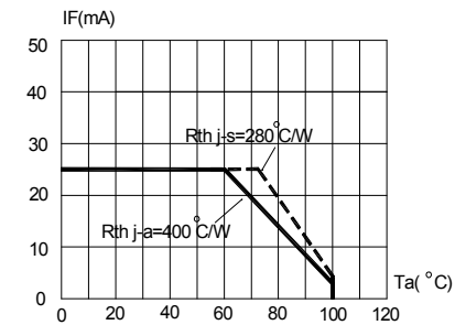
FIG.4b GREEN MAXIMUM FORWARD DC CURRENT VS AMBIENT TEMPERATURE ( T_{jmax}=110^{\circ}C )
